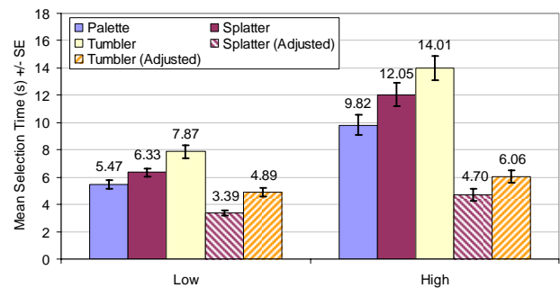
Figure 6: Complexity vs. Selection Trial Time by Tool.
